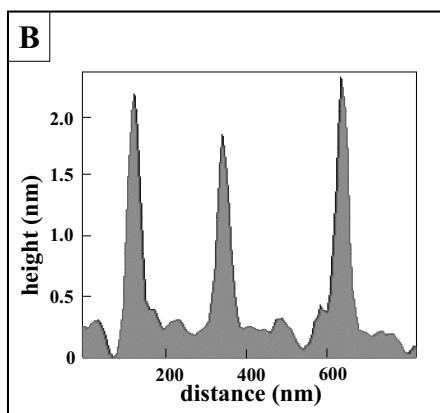
(A) A 1.7x 1.7 \mu\text{m}^2 topographic image. (B) Corresponding cursor profile for the line shown in (A). The cursor profile shows the diameters of the three particles are 2.0 nm, 1.6 nm and 2.1 nm, respectively.
