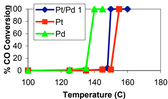
Figure 2. Kinetic study of CO oxidation.
