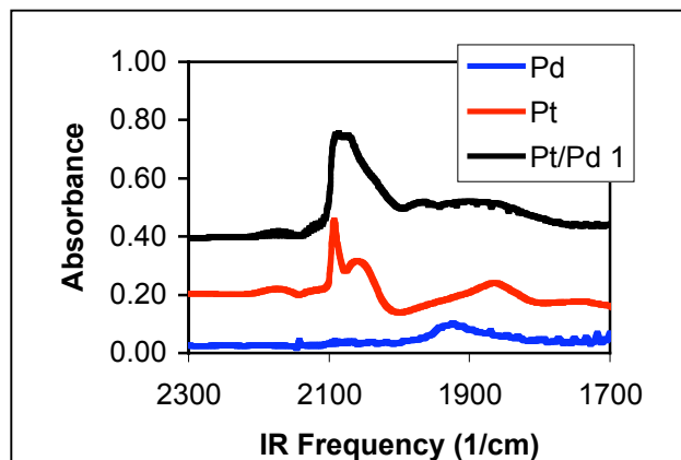
Figure 1. IR spectra of CO adsorbed on dendrimer-templated catalysts.
