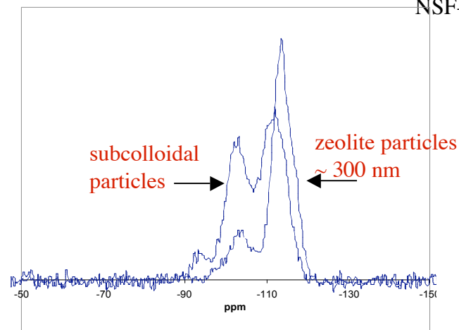
Figure 2. 29 Si MAS NMR of silicalite-1 subcolloidal particles and 300 nm zeolite particles.
